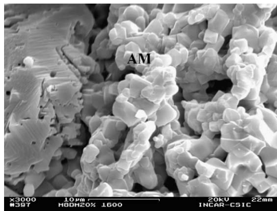
Fig. 7. Spinel crystals (AM) in the 8DM20% matrix composition at 1600 °C.
